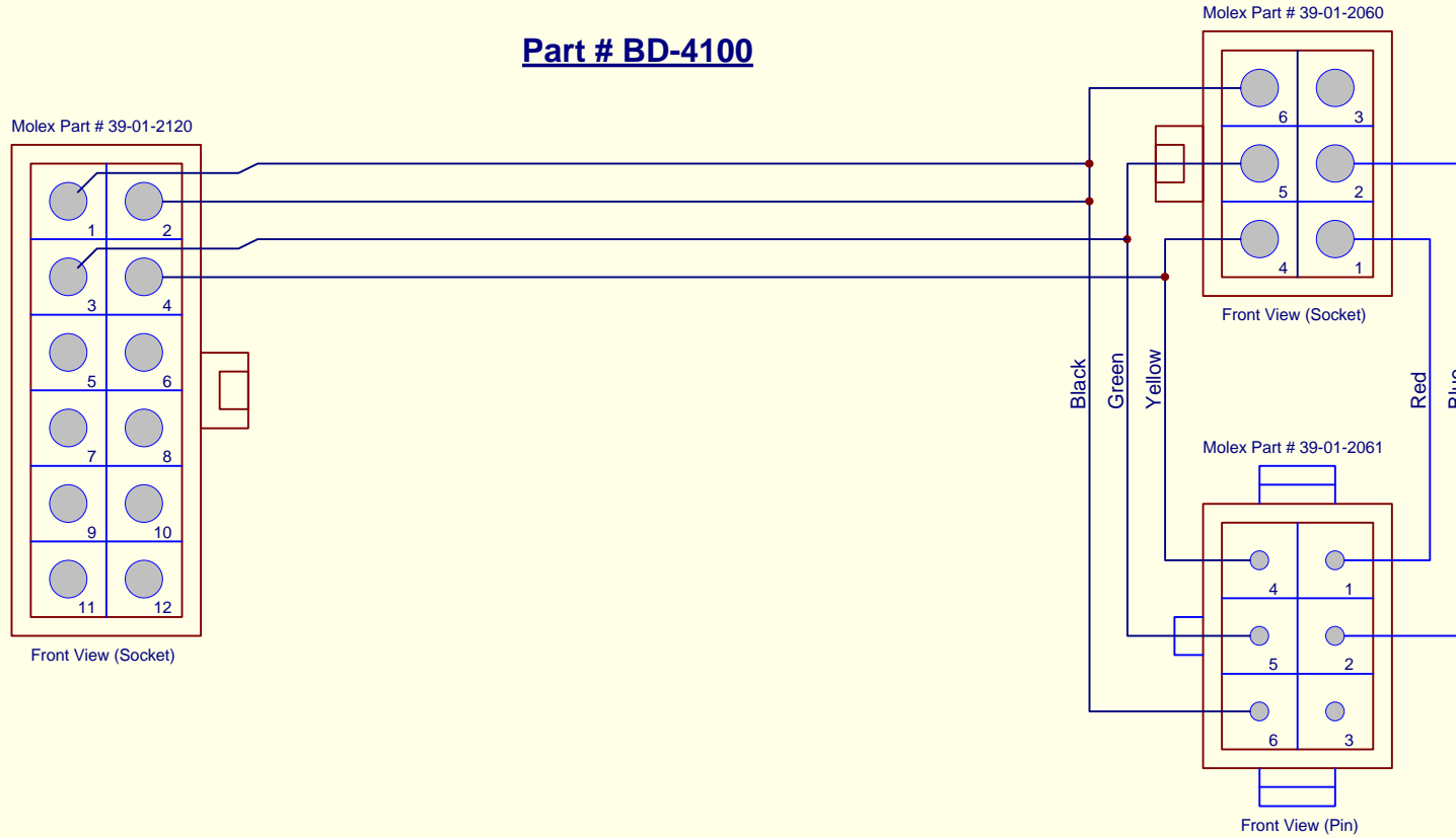
Fron view X1 of interface
